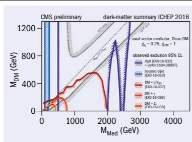
Fig. 1. (Left) 95% CL exclusion regions in the mass plane of the mediator and DM candidate for dijet searches and different values of ETmiss.
