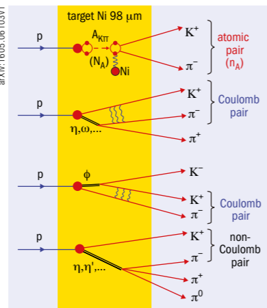
Inclusive \pi K production via the interaction p + Ni \rightarrow \pi K + X . The ionisation or break up of A_{K\pi} leads to so-called atomic pairs.
