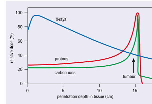
Effective relative dose versus tissue depth for different forms of radiation.
