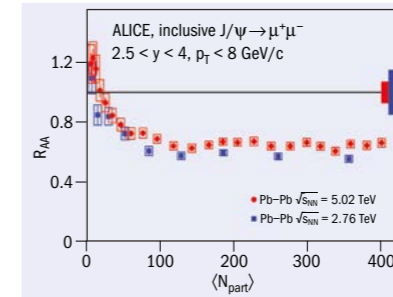
The J/ψ nuclear modification factor versus the average number of nucleons participating in Pb-Pb collisions at nucleon-nucleon collision energies of 5.02 (red) and 2.76 (blue) TeV.
