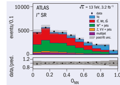
The neural-network discriminant for the positive lepton channel in the signal region. The signal and backgrounds are normalised to the fit results and the hatched and grey histograms represent the uncertainty.
