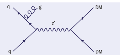
Fig. 2. (Below) Feynman diagrams showing the production of the mediator and its decay to SM (left) and DM (right) particles. The former yields a dijet topology while the latter produces events with a high-momentum jet in combination with significant missing transverse energy.
