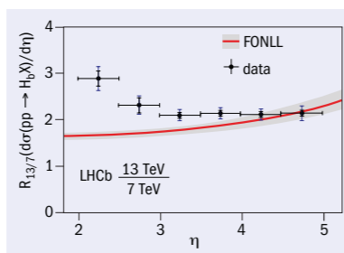
The ratio of differential cross-sections for b -hadron production with respect to pseudorapidity, \eta , measured at collision energies of 13 and 7 TeV. Data are compared to predictions described in Eur. Phys. J C 75 610.
