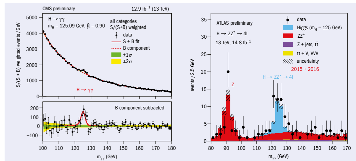
Fig. 2. In case there was any doubt about the existence of the Higgs boson, the CMS (left) and ATLAS (right) experiments have rediscovered the 125 GeV-mass particle in independent data recorded at almost twice the collision energy (13 TeV).
