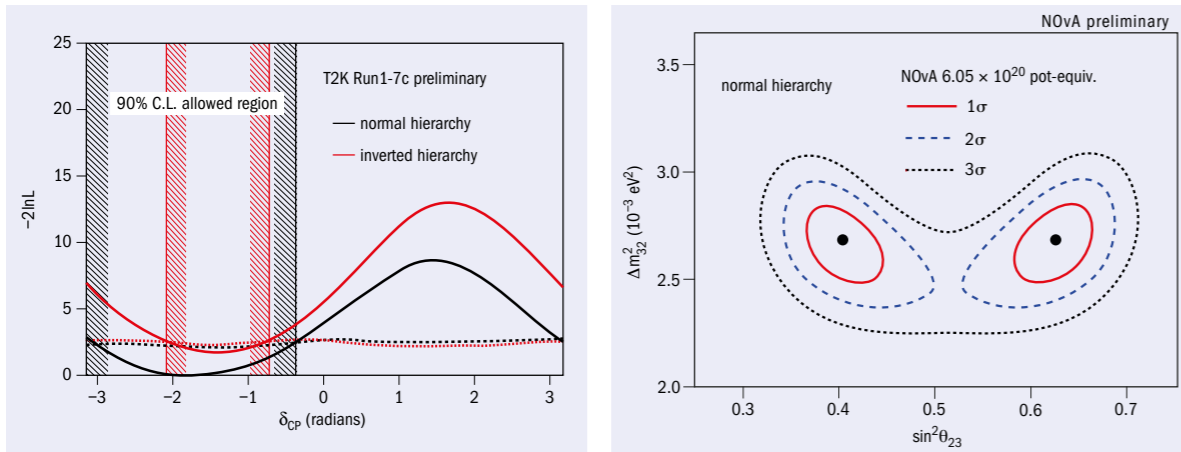
Fig. 3. With nearly twice the antineutrino data in 2016 compared with its 2015 result, the T2K experiment's observed electron antineutrino appearance rate is lower than would be expected if CP asymmetry is conserved (left). With data accumulated until May 2016, representing 16% of its planned total, NOvA's results (right) show an intriguing preference for non-maximal mixing – that is, a preference for \sin^2\theta_{23} \neq 0.5 .
