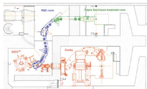
The S2C2 cyclotron and its compact gantry produced by IBA. Blue shows the beamline that feeds the R&D room for the France Hadron research teams, while green shows the second fixed-beam treatment room, which will be installed in the near future.
