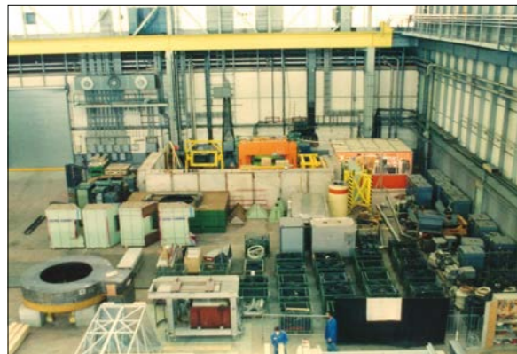
The MEDICYC Cyclotron (the orange magnet in the back) in the PS East Hall during tests in the early 1990s.
